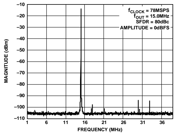
Figure 24. Single-Tone SFDR
