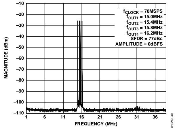
Figure 26. Four-Tone SFDR
