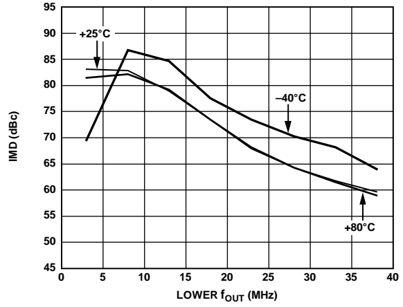
Figure 37. Dual-Tone IMD vs. Lower f_{OUT} and Temperature at 80 MSPS, I_{OUTFS} = 2 \text{ mA} and 0 dBFS
